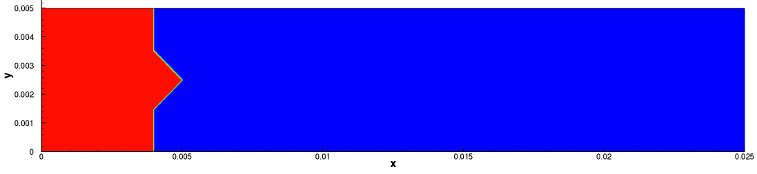
Figure 16: Schematic of the 2D detonation test case initial data.
