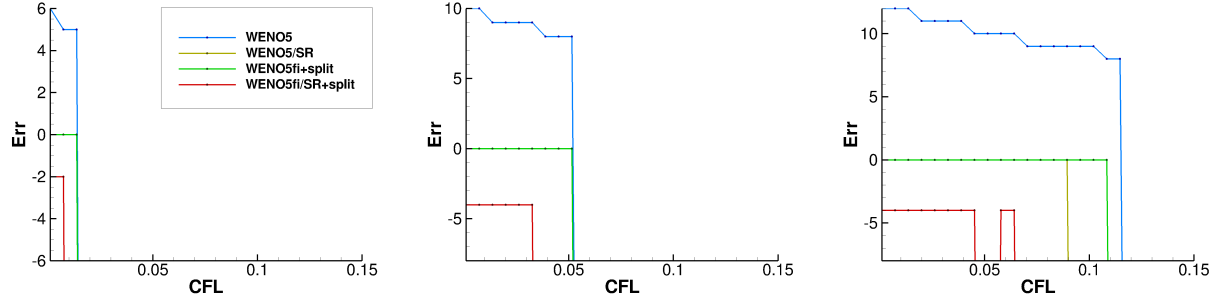
Figure 13: No cutoff safeguard procedure and Strang splitting results for the 1D C-J detonation problem, Arrhenius case at t = 1.8 : Number of grid point away from the reference shock solution (Err) as a function of the CFL number (128 discrete CFL values with 6.316455696 \times 10^{-3} equal increment) for three low dissipative shock-capturing methods using 50, 150, 300 uniform grid points (across) and for stiffness K_0 .
