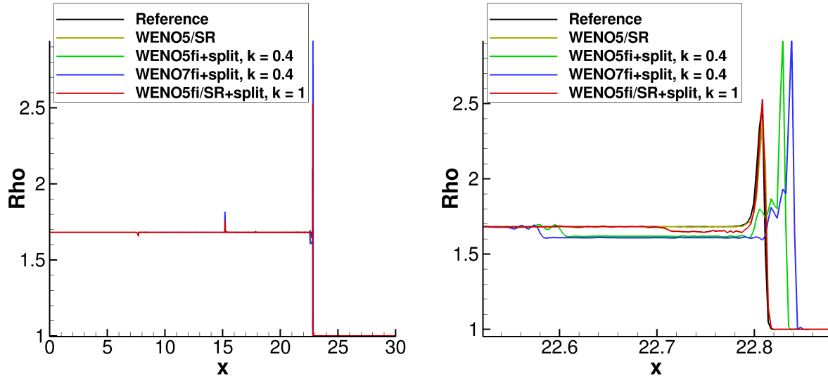
Figure 22: 1D C-J detonation problem, Arrhenius case at t = 1.8 : Behavior of WENO5/SR, WENO5fi+split and WENO5fi/SR+split under extreme grid refinement with CFL = 0.05 and 10,000 grid points. The value "k" is the \kappa value to control the amount of numerical dissipation indicated in the formula for the filter numerical fluxes [26].
