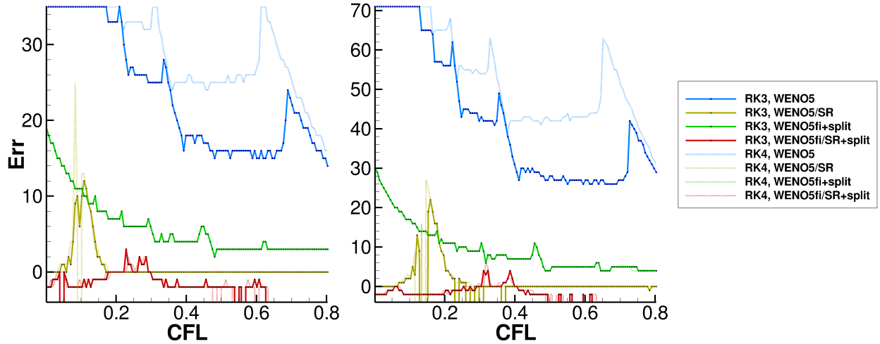
Figure 14: 1D C-J detonation problem, Arrhenius case at t = 1.8 : Comparison of the same spatial discretization with RK4 and RK3 temporal discretization for three low dissipative shock-capturing methods using 150, 300 uniform grid points and for stiffness K_0 .
