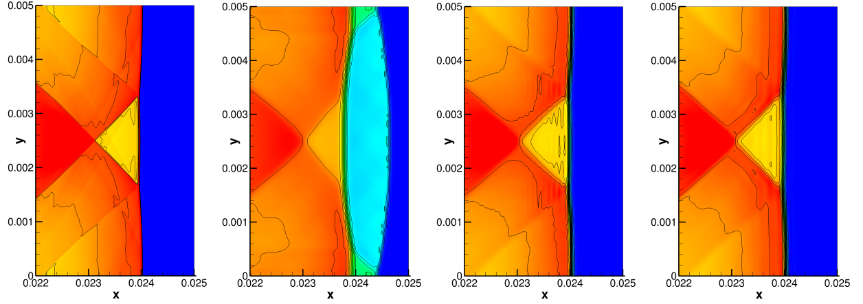
Figure 18: 2D detonation problem at t = 1.7 \times 10^{-7} and K_0 = 0.5825 \times 10^{10} : Density computed by different methods. From left to right: reference solution by the standard WENO5 method using 4000 \times 800 uniform grid points, WENO5, WENO5/SR and WENO5fi+split using 500 \times 100 uniform grid points with CFL = 0.05 .
