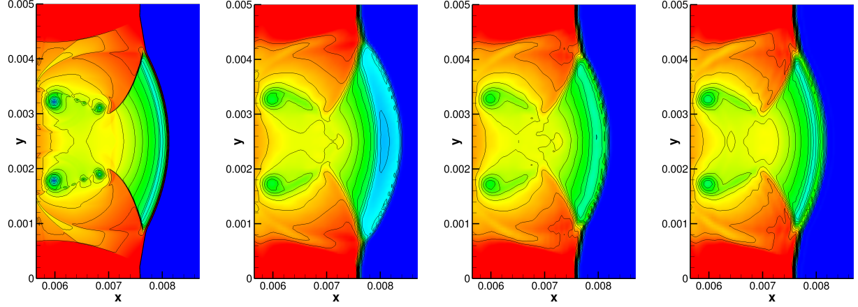
Figure 17: 2D detonation problem at t = 0.3 \times 10^{-7} and K_0 = 0.5825 \times 10^{10} : Density computed by different methods. From left to right: reference solution by the standard WENO5 method using 4000 \times 800 uniform grid points, WENO5, WENO5/SR and WENO5fi+split using 500 \times 100 uniform grid points with CFL = 0.05
