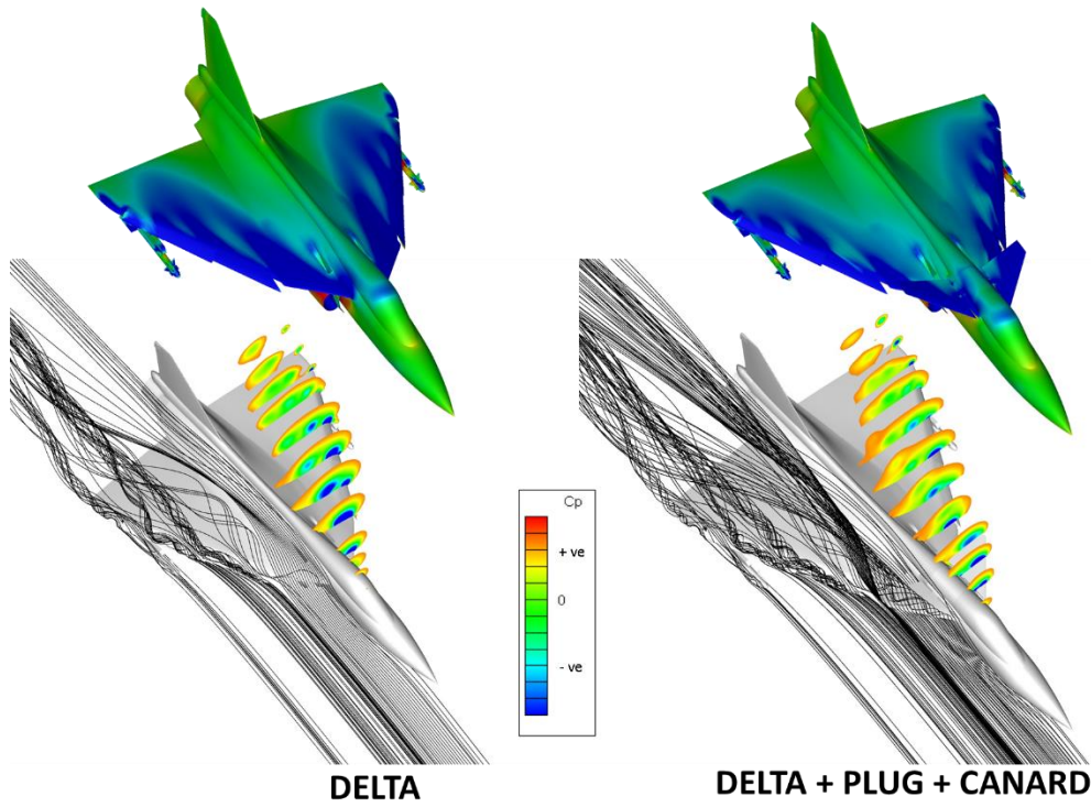
Figure 8: Surface pressure contours from CFD for DELTA and DELTA+PLUG+CANARD for \text{AOA}=18^\circ .
