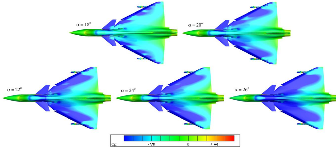
Figure 7: Surface pressure contours from CFD for DELTA+PLUG+CANARD configuration.
