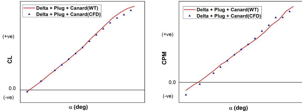
Figure 4: CFD and Wind tunnel results for the DELTA+PLUG+CANARD configuration.
