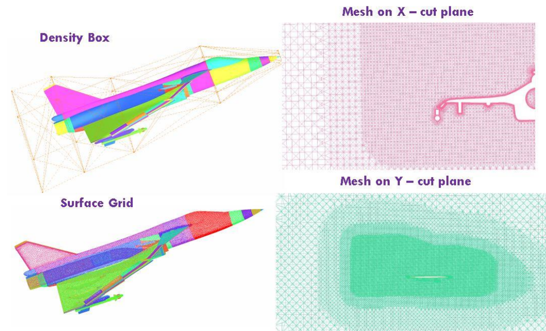
Figure 3: Basic grid details used for the CFD studies.
