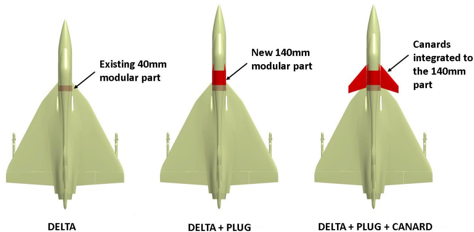
Figure 1: Three configurations tested in Wind tunnel (1:10 scale).
