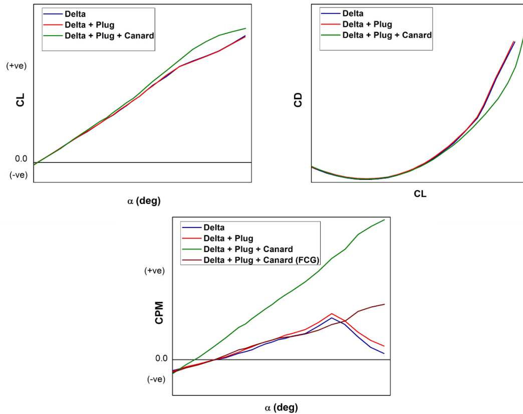
Figure 6: Basic aerodynamic characteristics with full slat deflections from Wind tunnel tests.
