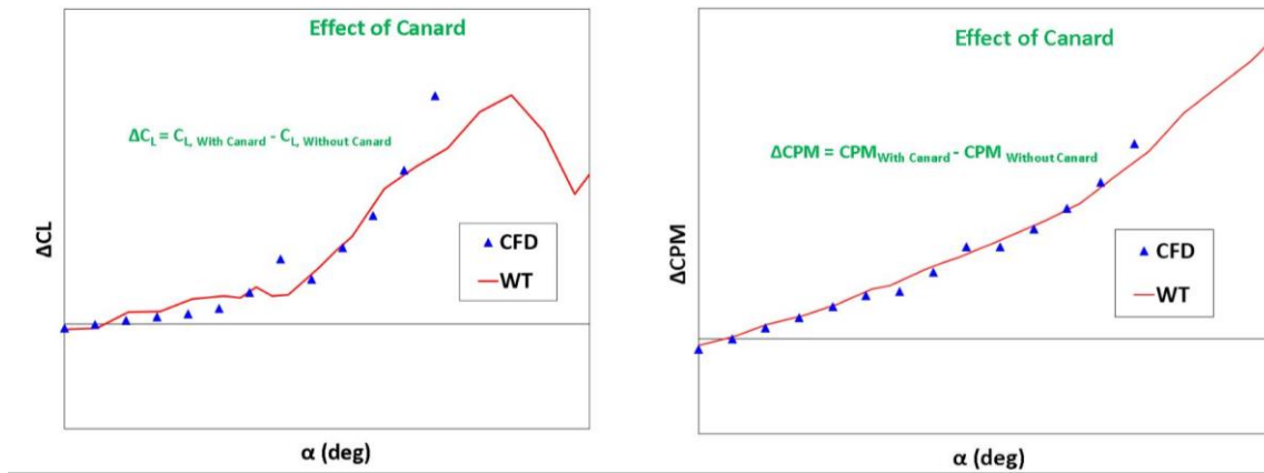
Figure 5: CFD and Wind tunnel results of the delta effect of canard.
