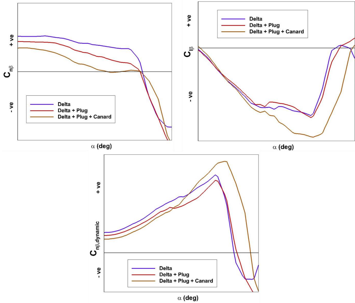
Figure 9: Lateral directional characteristics from Wind tunnel tests.
